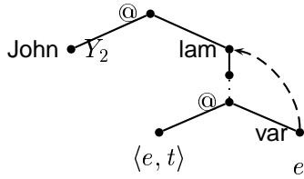
Figure 5: The elliptic sentence John did, too
