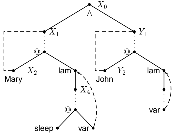
Figure 1: The parallelism constraint for the elliptical sentence in (4)
